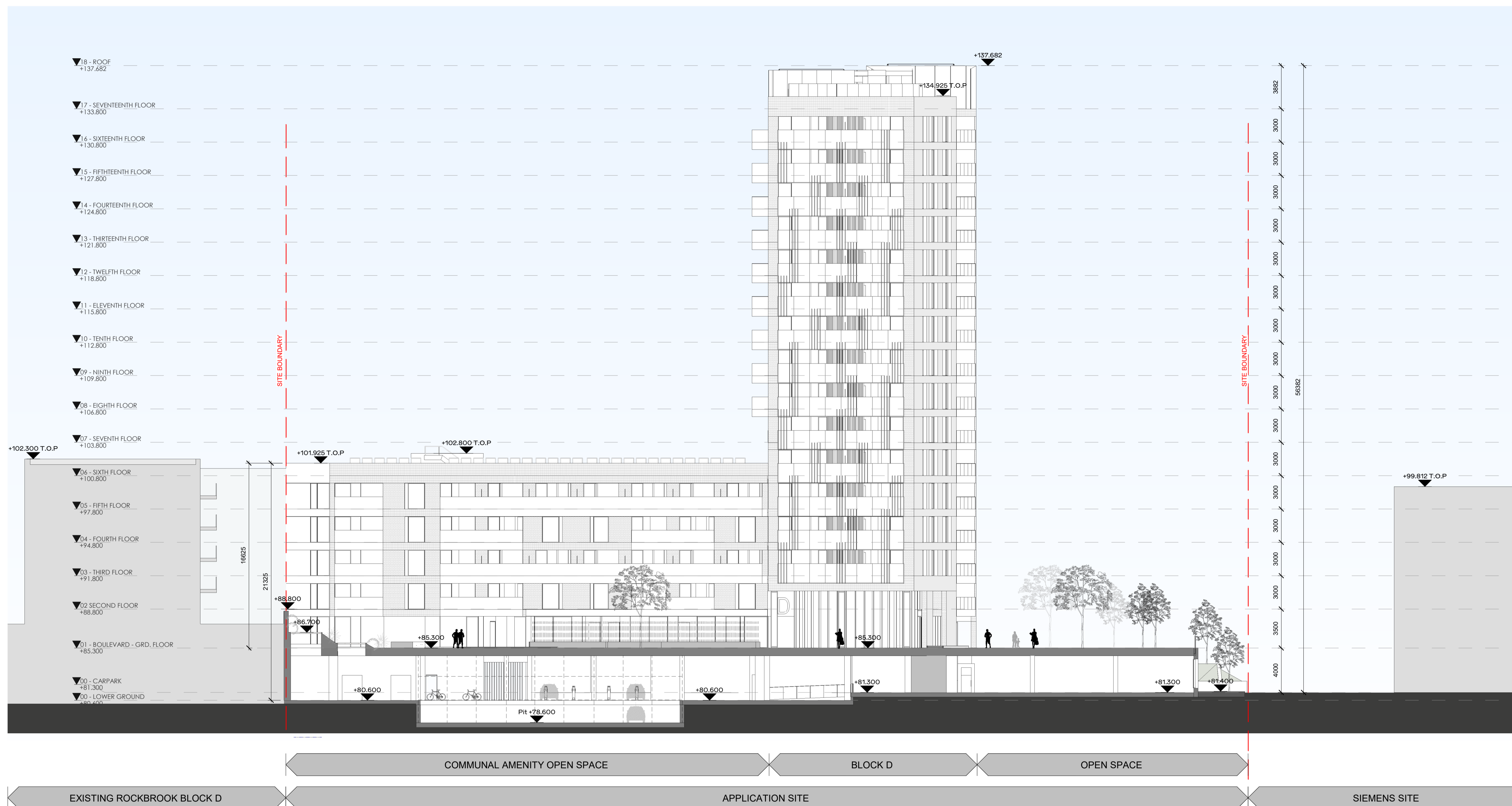
03 Section 03 1:200
